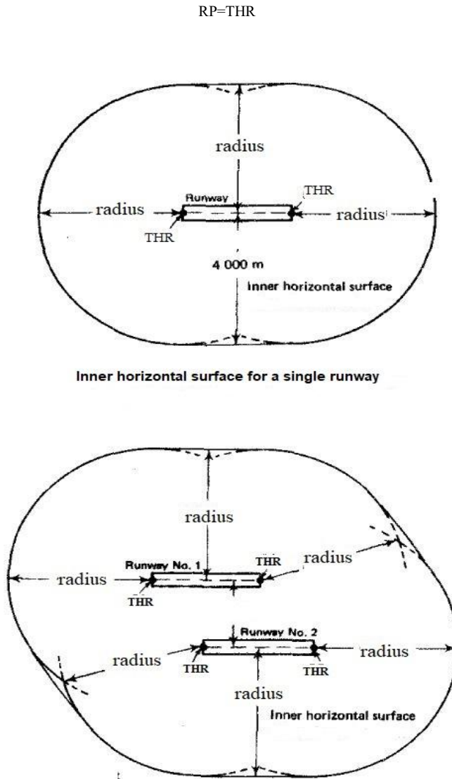
Figure G-2. Boundary of inner horizontal surface (illustrates matters)
