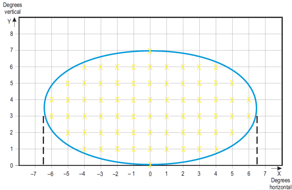
Figure AH-16. Grid points to be used for calculation of average intensity of approach and runway lights
