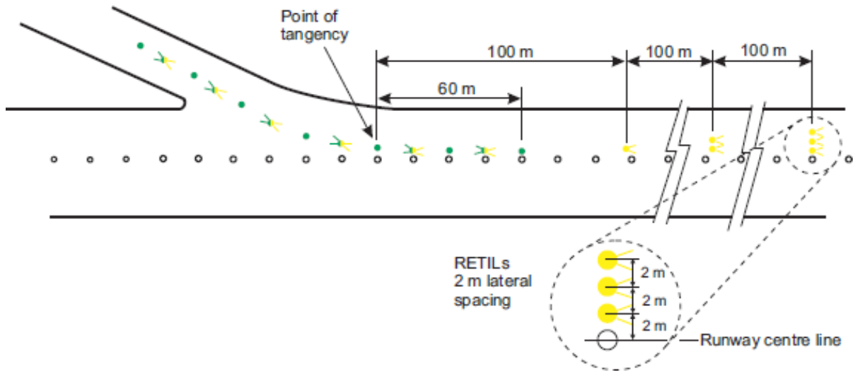
Figure H-22. Rapid exit taxiway indicator light (RETILs)
