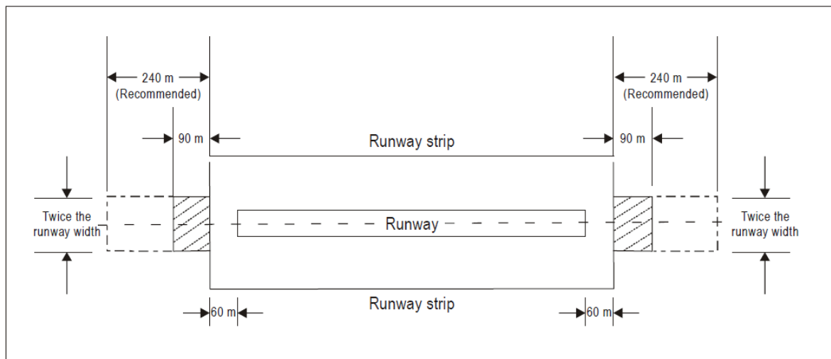
Figure AF-4 (1). Runway end safety area for a runway where the code number is 3 or 4
