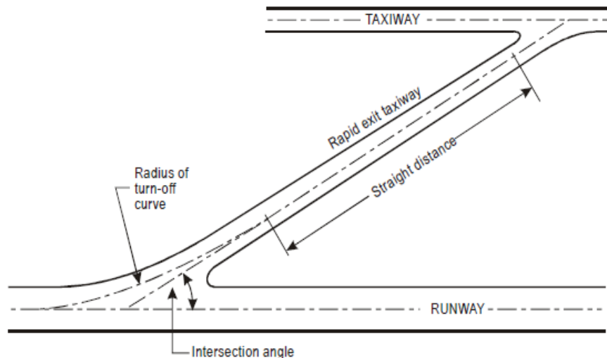
Figure F-3. Rapid Exit Taxiway
