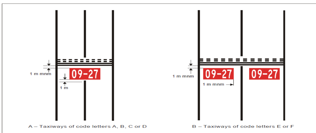
Figure H-10. Mandatory instruction marking.
